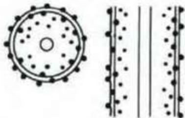
(2) Parts of cuticle and cortex (Semi-permanent hair color)
